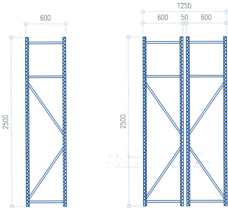
SIDE ELEVATION
